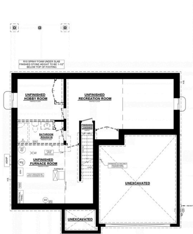
BRIARWOOD A BASEMENT PLAN
