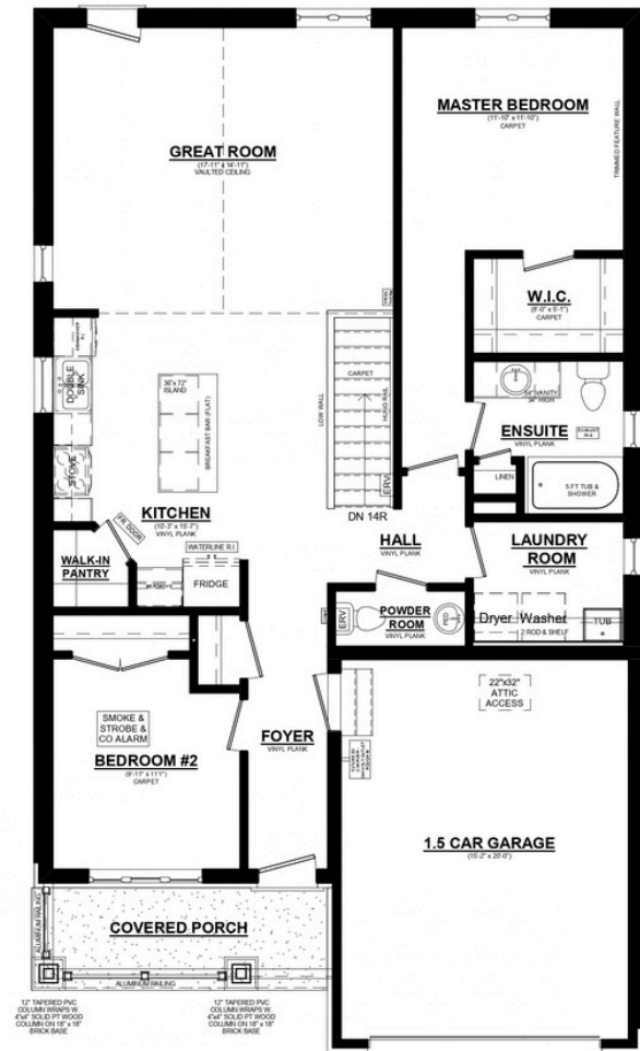
GLENWOOD C MAIN FLOOR PLAN 1276 SQ. FT. 8' CEILINGS ON MAIN FLOOR
