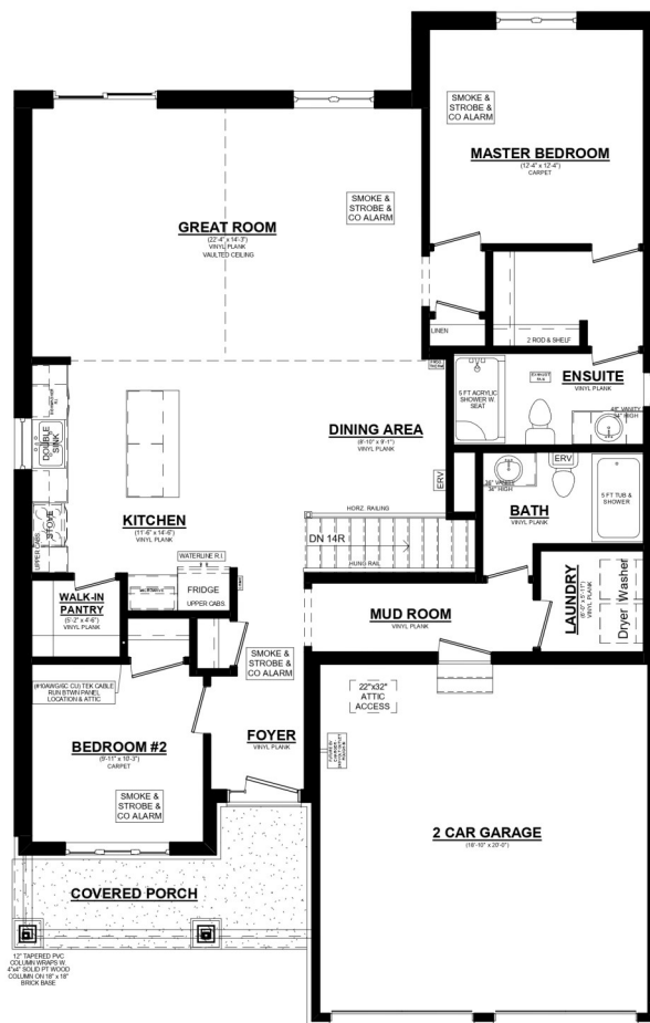
ROSEWOOD A MAINFLOOR PLAN 1440 SQ. FT. 8' CEILINGS ON MAINFLOOR
