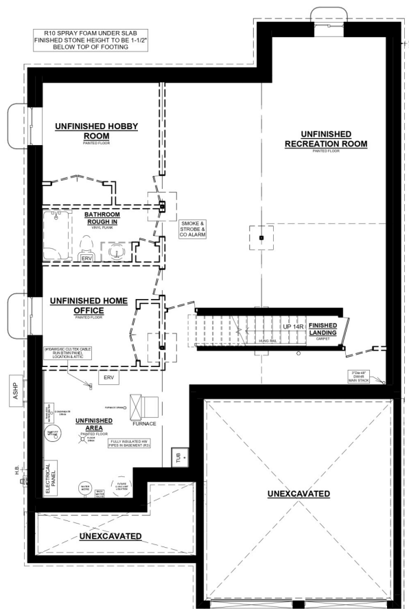
ROSEWOOD A BASEMENT PLAN
