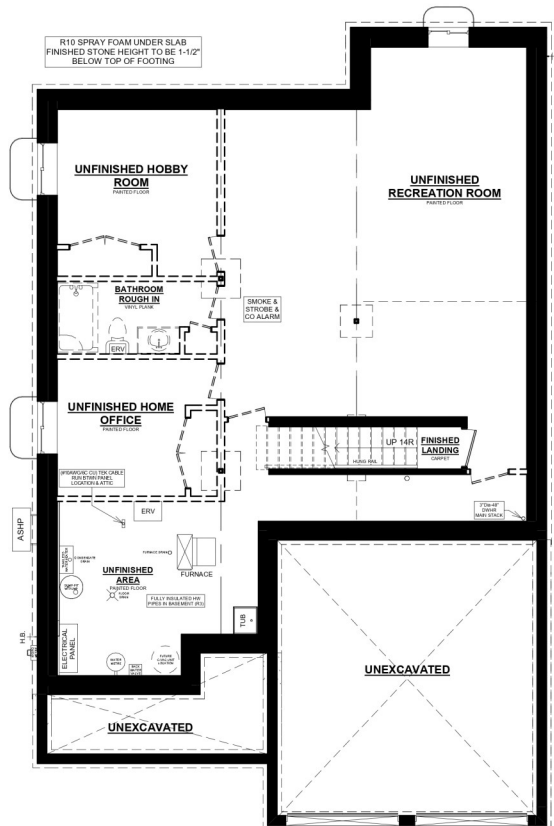
ROSEWOOD A BASEMENT PLAN
