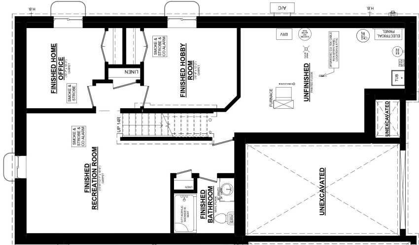
VALLEYBROOK D UNIT #2 BASEMENT PLAN 647 SQ. FT. FINISHED BASEMENT SPACE
