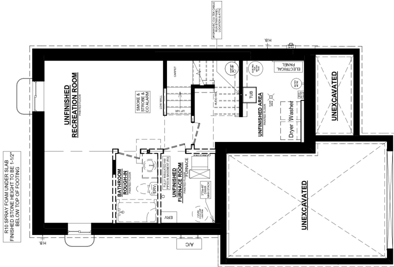
ASPEN 'A' BASEMENT PLAN
