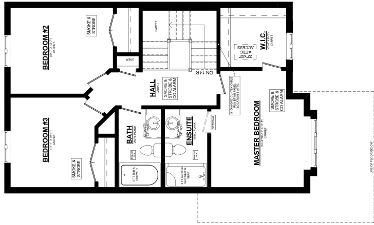
ASPEN 'A' 2ND FLOOR PLAN 775 SQ. FT. 2ND FLOOR
