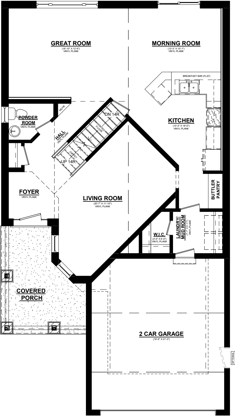
WINDFLOWER MAINFLOOR PLAN 1326 SQ. FT. 8' CEILINGS ON MAINFLOOR
