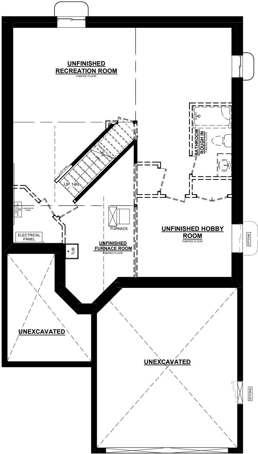
WINDFLOWER BASEMENT PLAN
