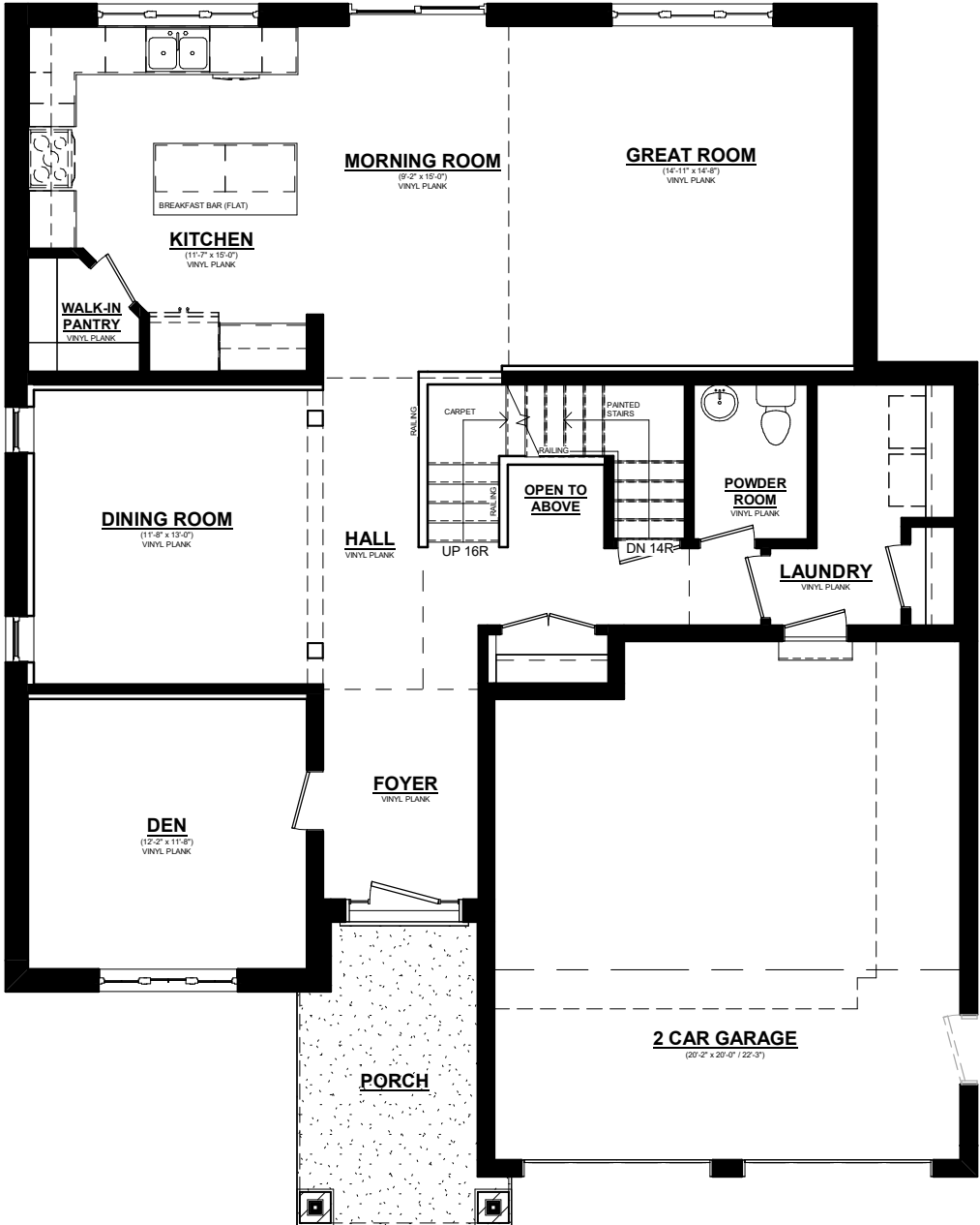
WILLOW MAINFLOOR PLAN 1389 SQ. FT. 9' CEILINGS ON MAINFLOOR
