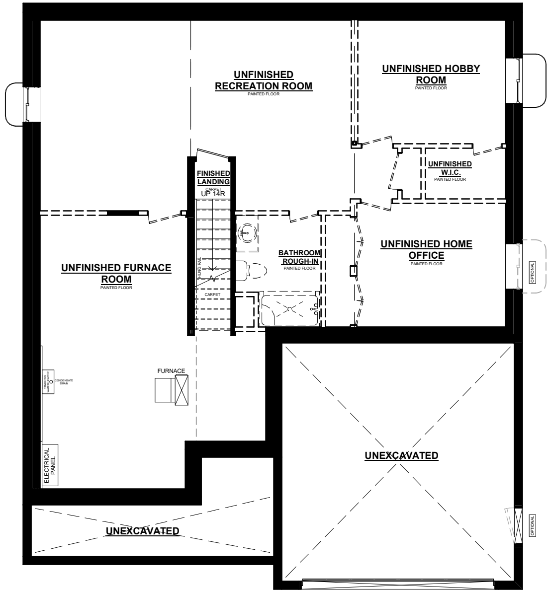
THORNWOOD BASEMENT PLAN
