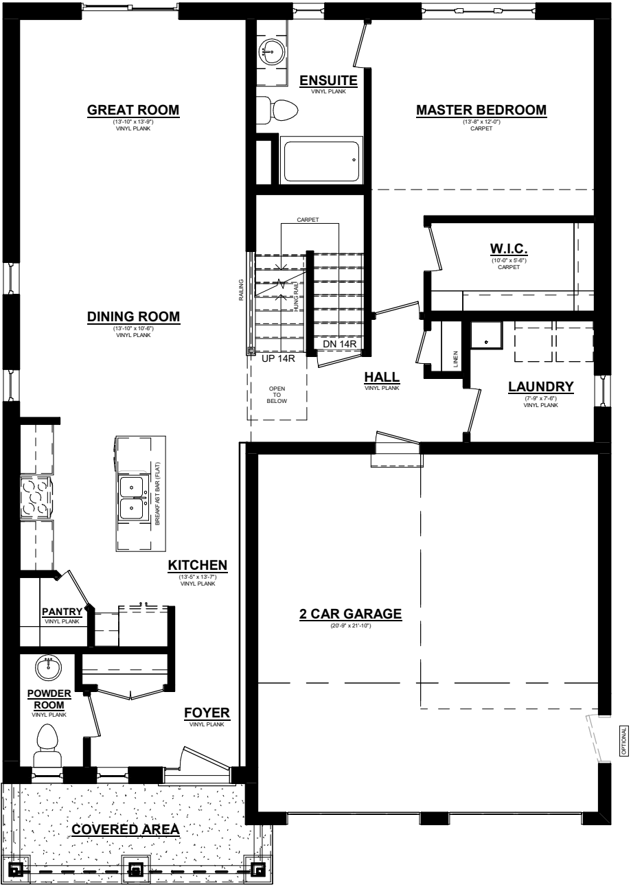
STONEHAVEN MAIFLOOR PLAN 1313 SQ. FT. 8' CEILINGS ON MAIFLOOR
