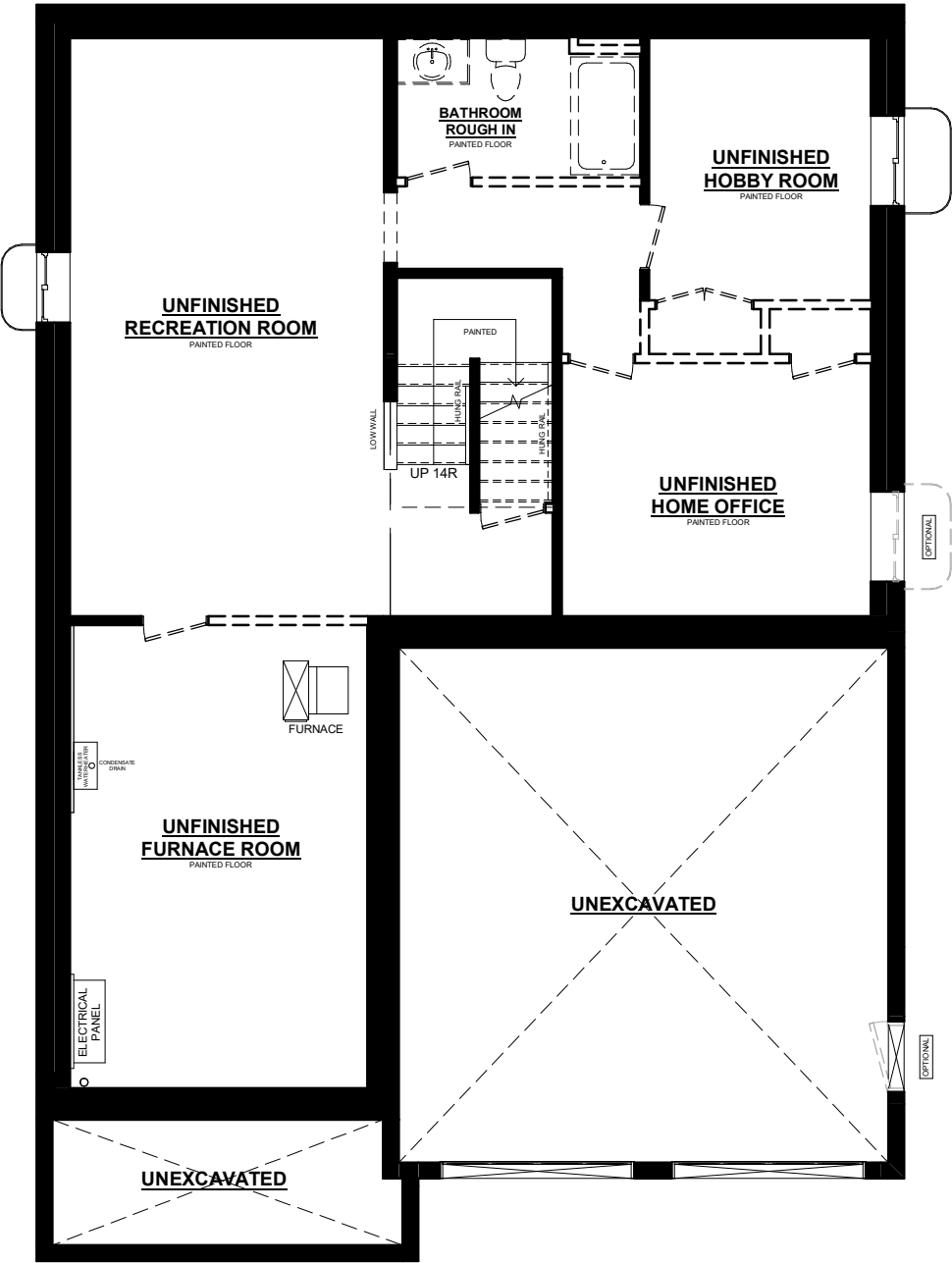
STONEHAVEN BASEMENT PLAN
