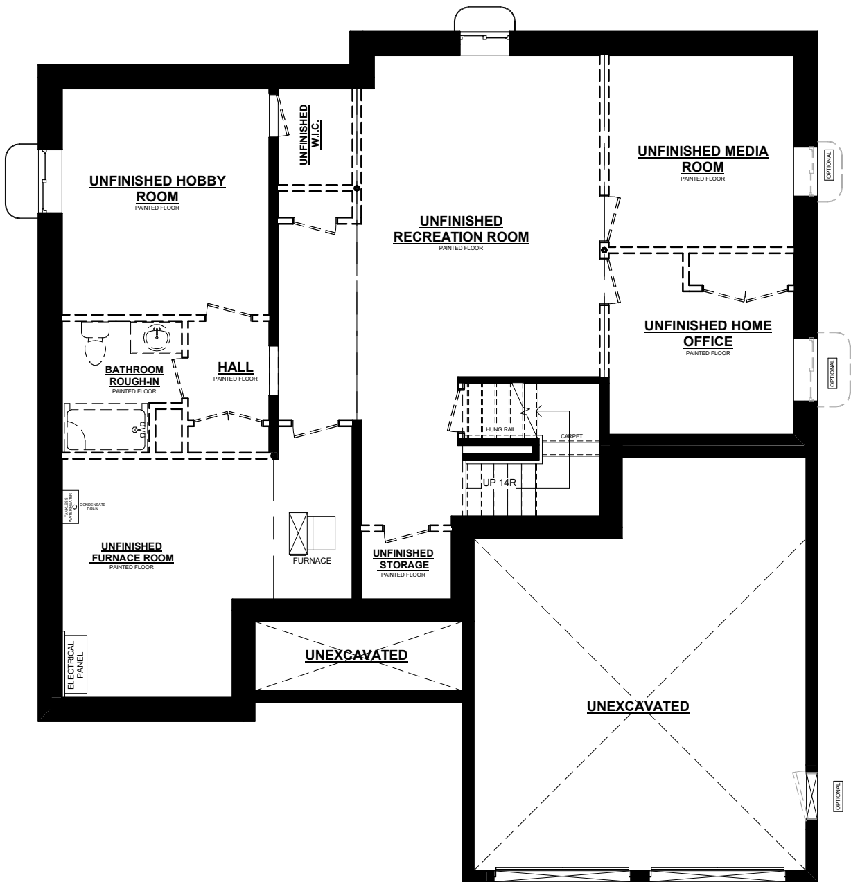
SOMERDALE BASEMENT PLAN
