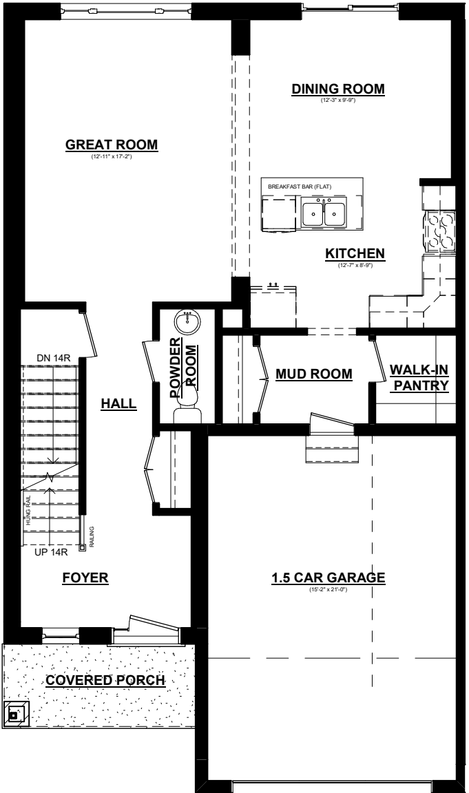
SEDONA MAIN FLOOR PLAN 879 SQ. FT. 8' CEILINGS ON MAIN FLOOR
