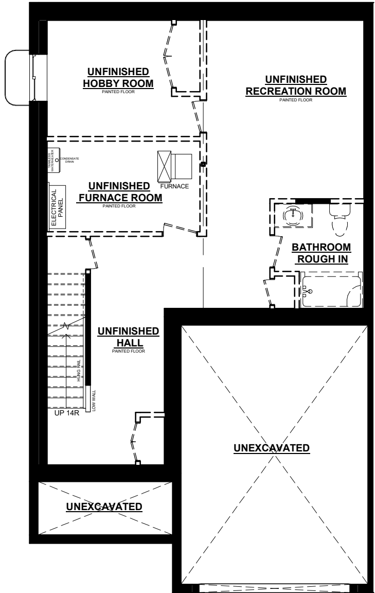
SEDONA BASEMENT PLAN
