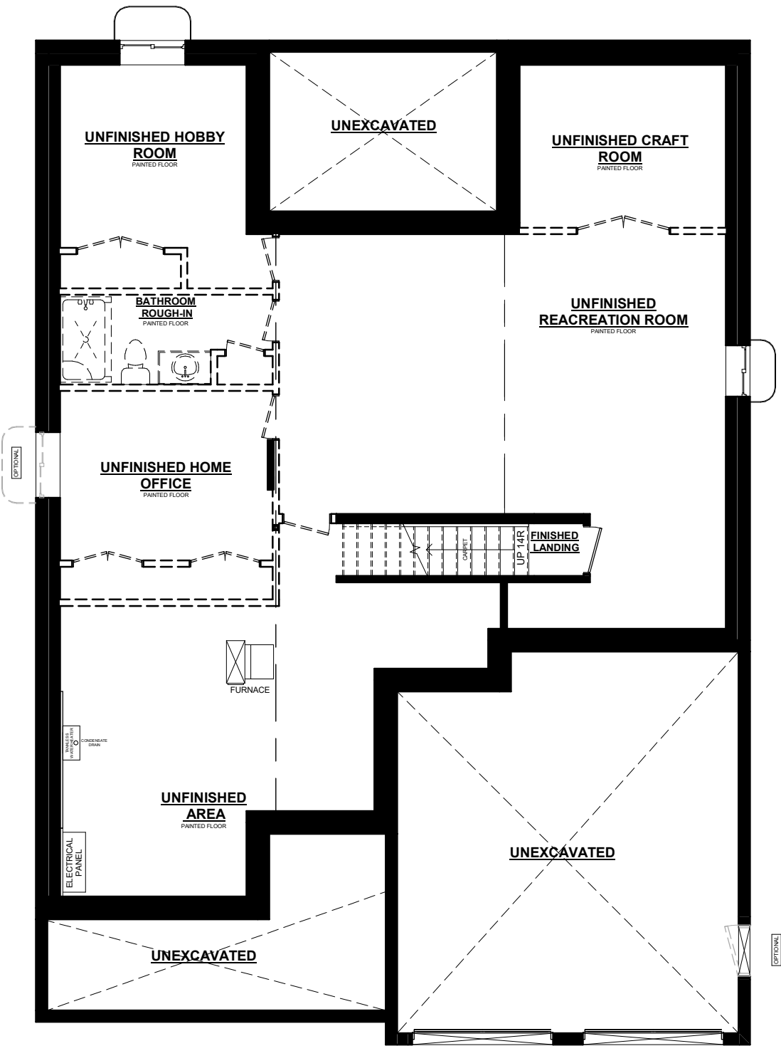
SAPPHIRE BASEMENT PLAN
