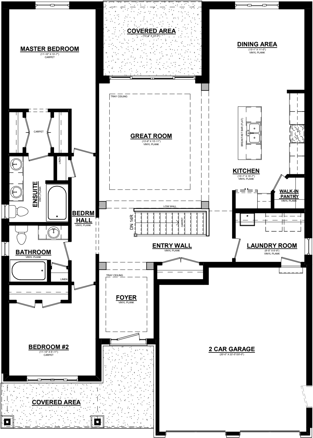
SAPPHIRE MAINFLOOR PLAN 1673 SQ. FT. 8' CEILINGS ON MAINFLOOR
