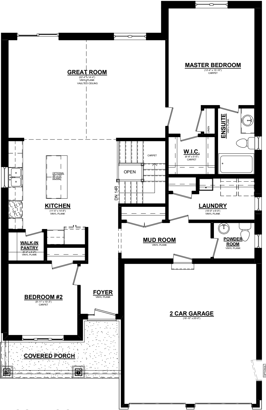
ROSEWOOD MAINFLOOR PLAN 1441 SQ. FT. 8' CEILINGS ON MAINFLOOR
