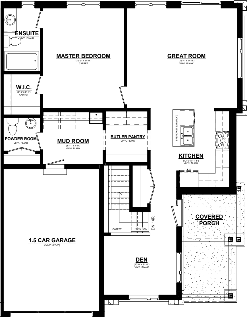
ROCKWOOD UNIT #2 MAIN FLOOR PLAN 1132 SQ. FT. 8' CEILINGS ON MAIN FLOOR
