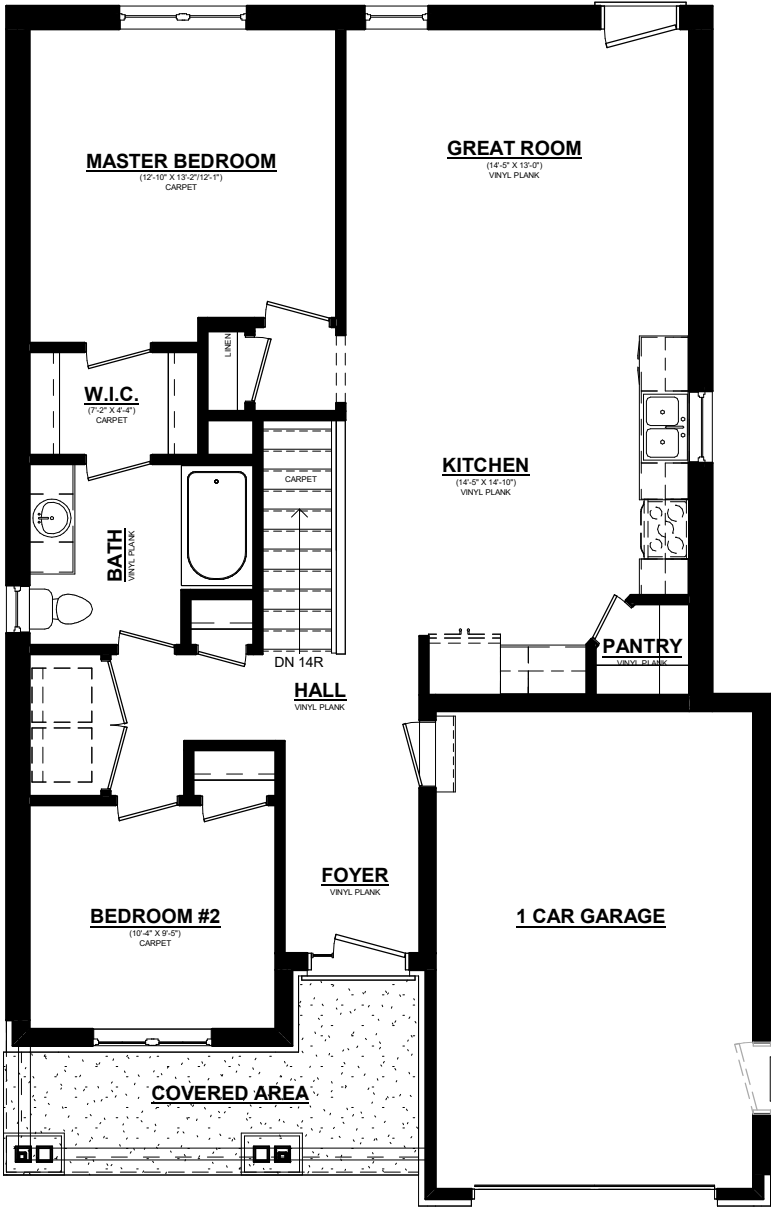
PINEWOOD MAINFLOOR PLAN 1100 SQ. FT. 8' CEILINGS ON MAINFLOOR
