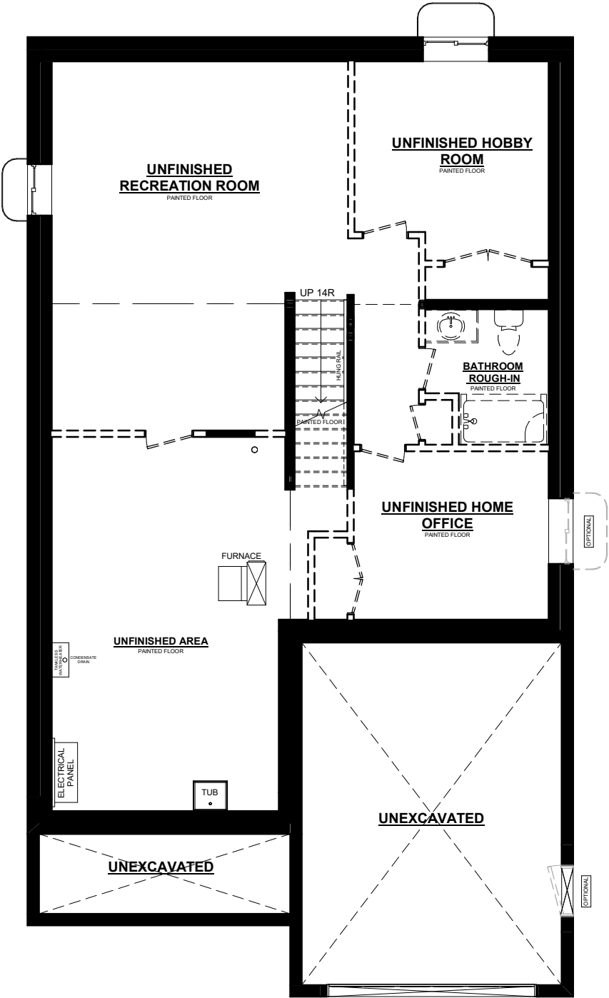
PALMER BASEMENT PLAN
