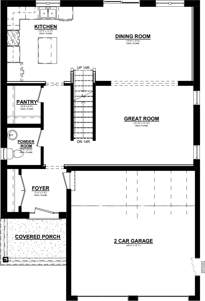
OAKMONT MAINFLOOR PLAN 948 SQ. FT. 8' CEILINGS ON MAINFLOOR
