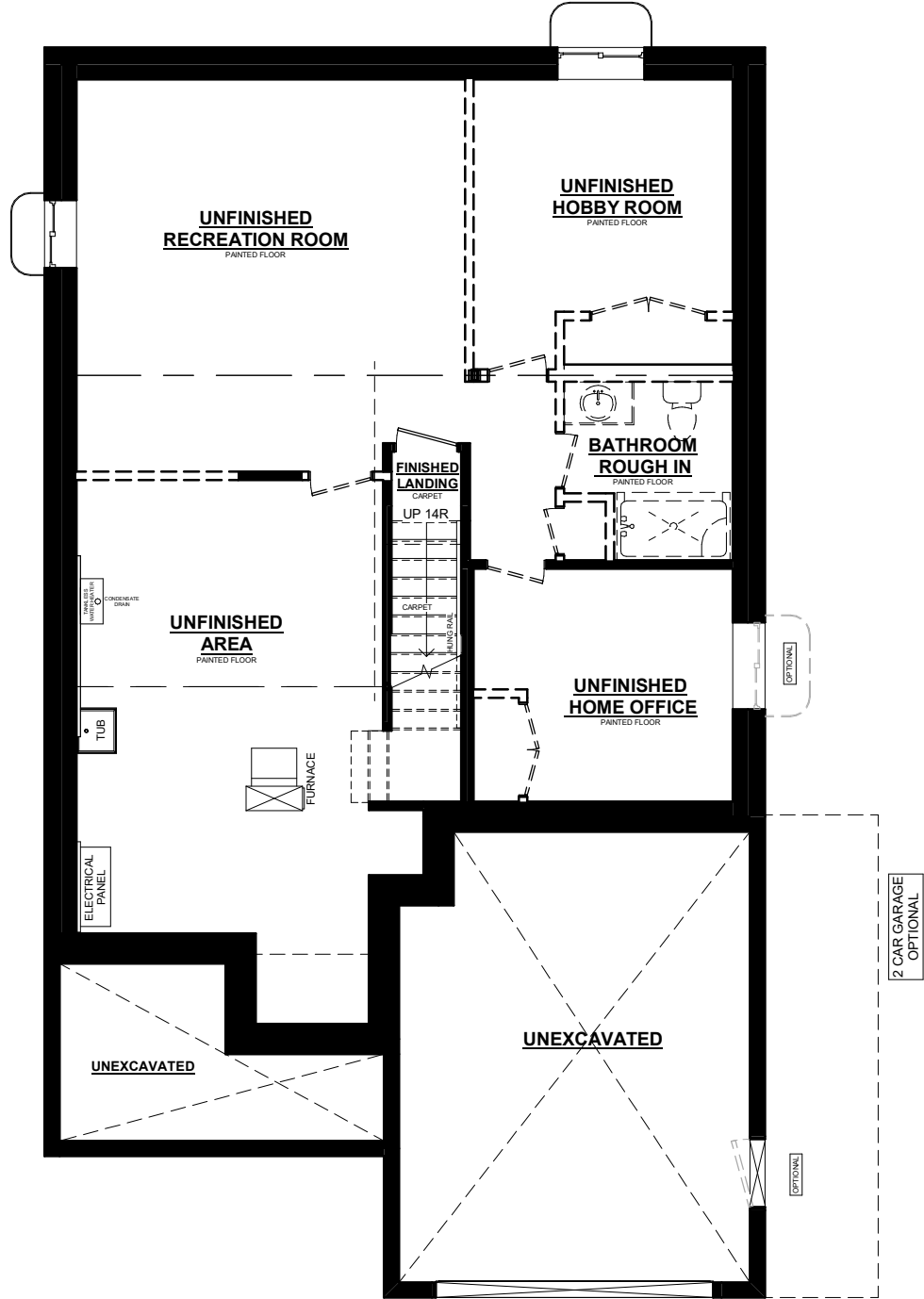
MAYFAIR BASEMENT PLAN
