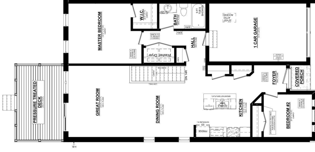
VALLEYBROOK D UNIT #1 MAIN FLOOR PLAN 1185 SQ. FT. 8' CEILINGS ON MAIN FLOOR
