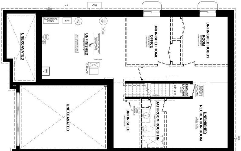
EASTON A UNIT #1 BASEMENT PLAN
