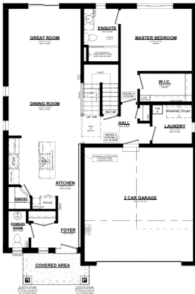
STONEHAVEN C MAIFLOOR ELEVATION 1313 SQ. FT. 8' CEILINGS ON MAINFLOOR
