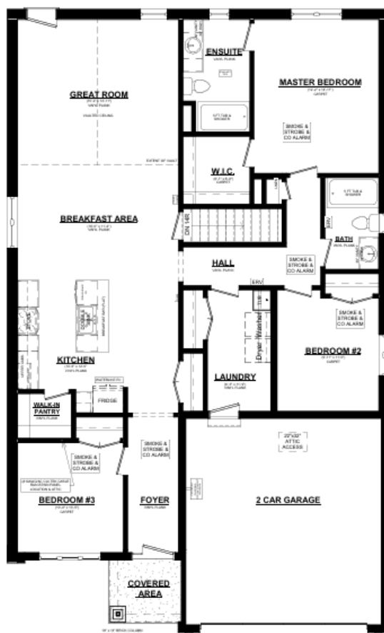
DUNMOOR C MAINFLOOR ELEVATION 1684 SQ. FT. 8" CEILINGS ON MAINFLOOR
