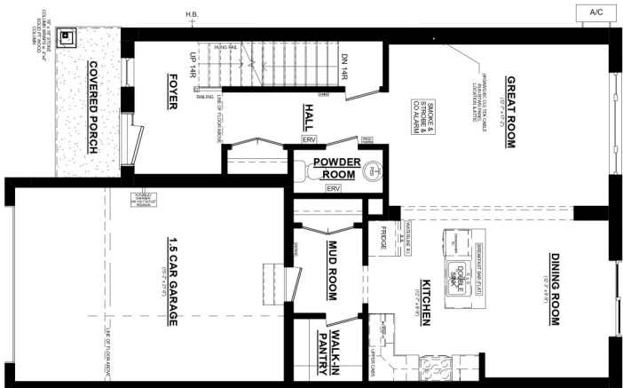
SEDONA 'A' UNIT #1 MAIN FLOOR PLAN 879 SQ. FT. 8' CEILINGS ON MAIN FLOOR
