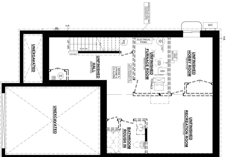
SEDONA 'A' UNIT #1 BASEMENT PLAN
