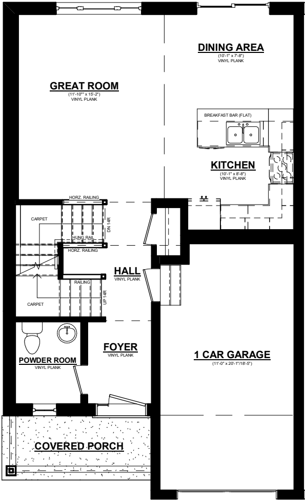
KENSINGTON MAIN FLOOR PLAN 650 SQ. FT. 8' CEILINGS ON MAIN FLOOR
