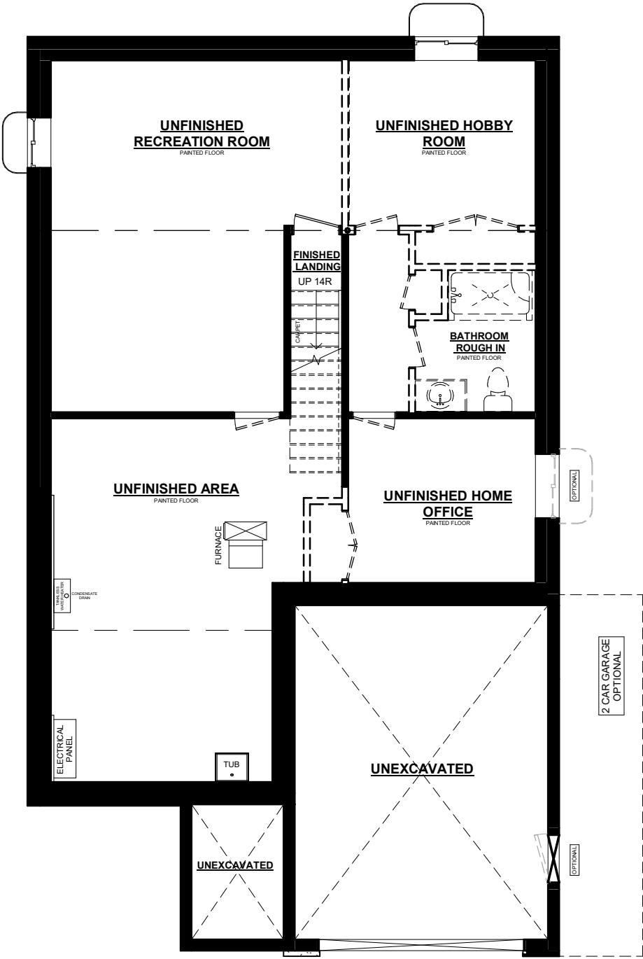
GLENWOOD BASEMENT PLAN
