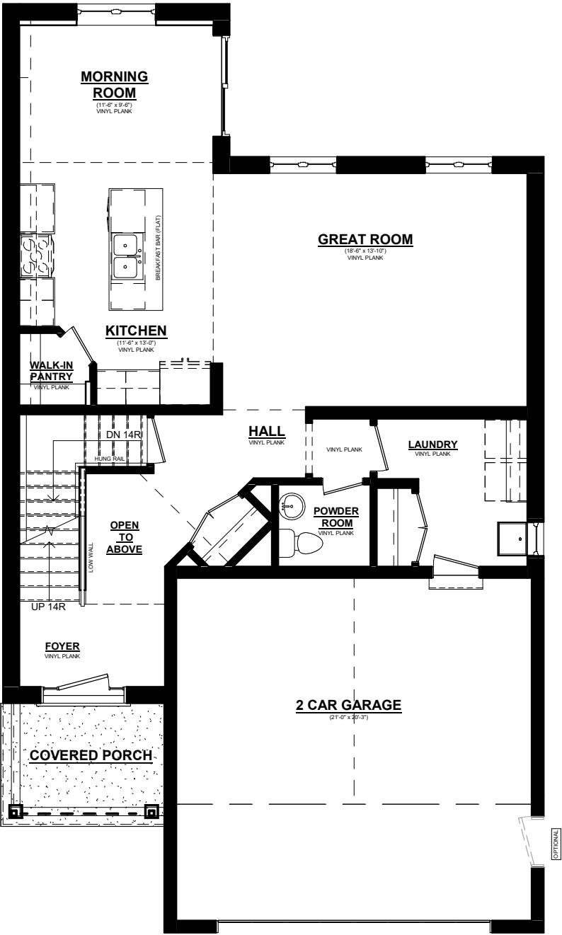
EDENBROOK MAINFLOOR PLAN
