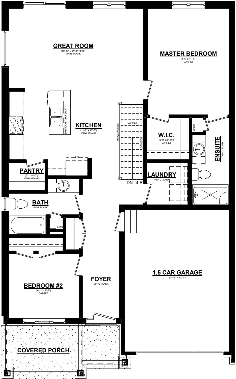
EASTON MAIN FLOOR PLAN 1200 SQ. FT. SQ. FT. 8' CEILINGS ON MAIN FLOOR
