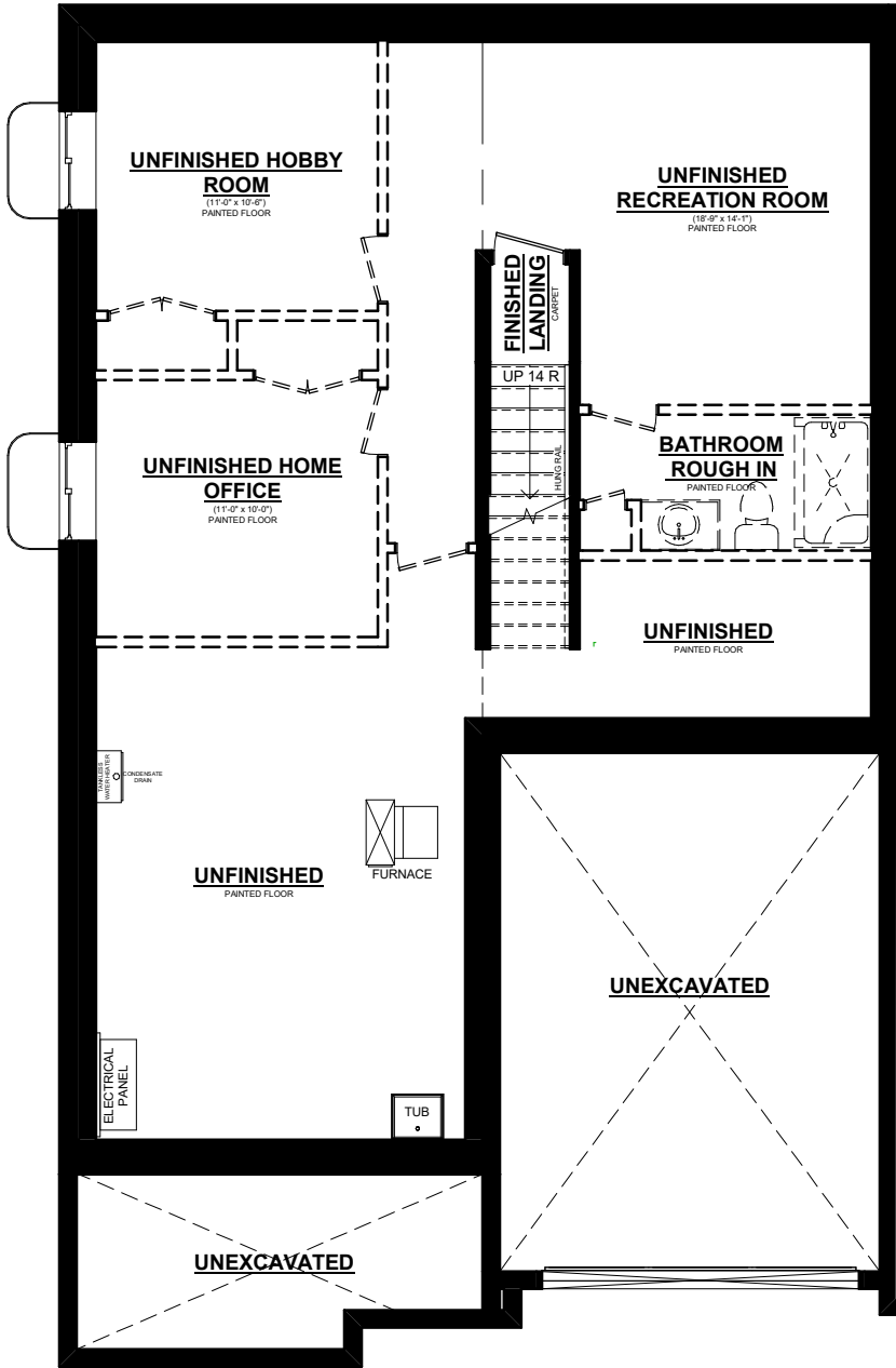
EASTON BASEMENT PLAN
