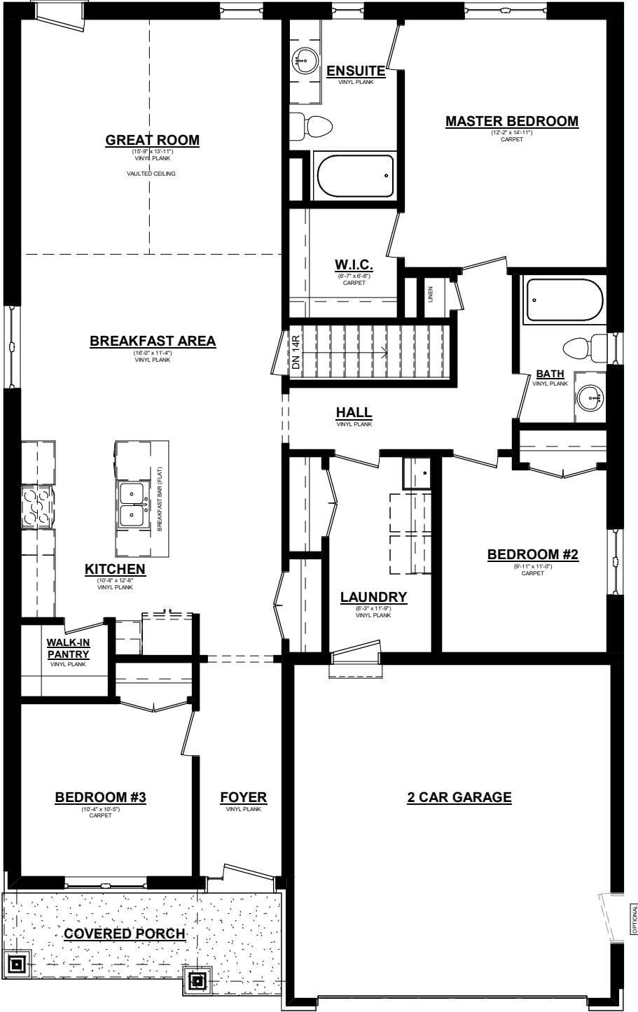
DUNMOOR MAINFLOOR PLAN 1684 SQ. FT. 8' CEILINGS ON MAINFLOOR
