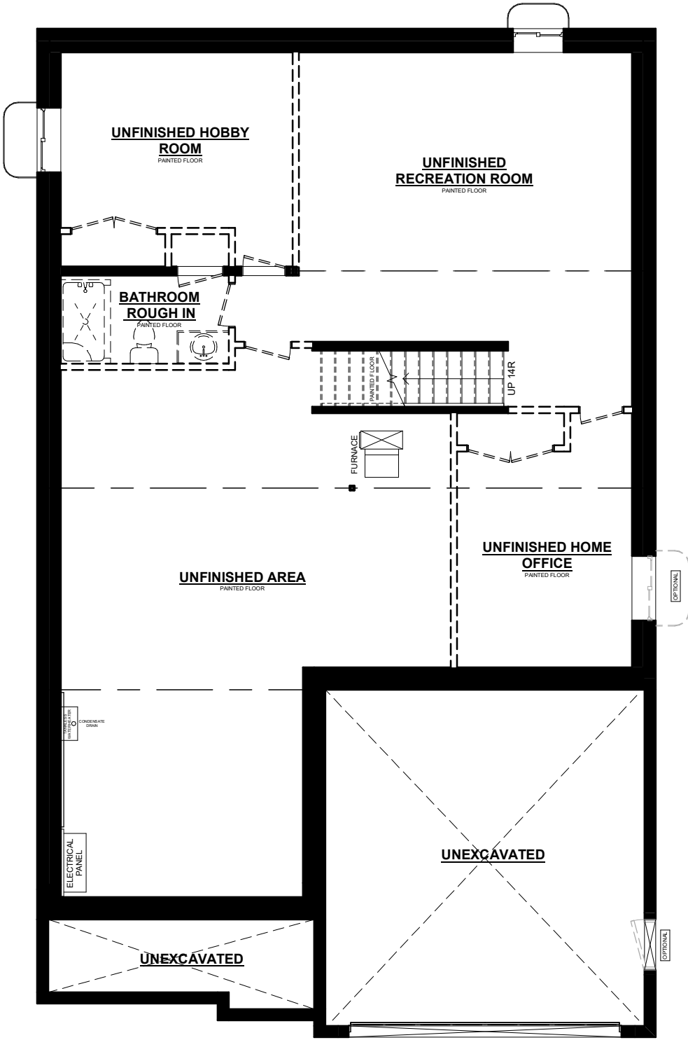
DUNMOOR BASEMENT PLAN
