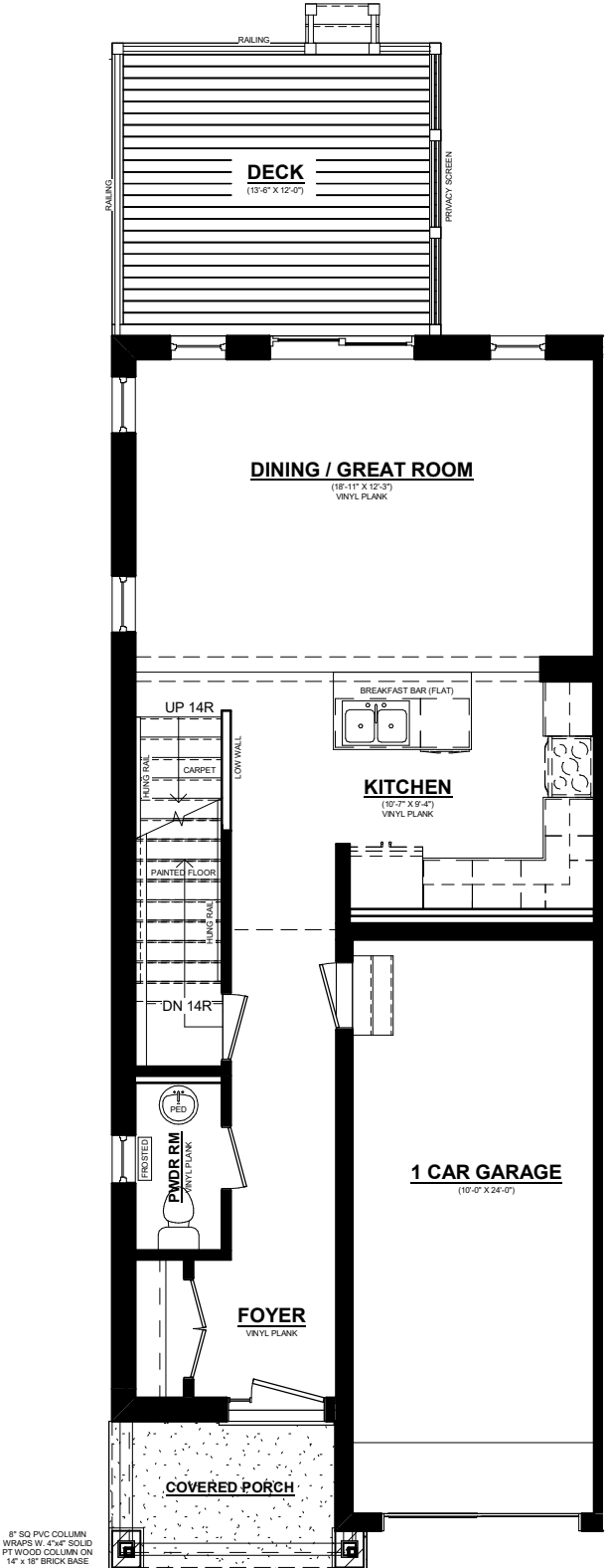
ASHTON MAINFLOOR PLAN 693 SQ. FT. 8' CEILINGS ON MAINFLOOR
