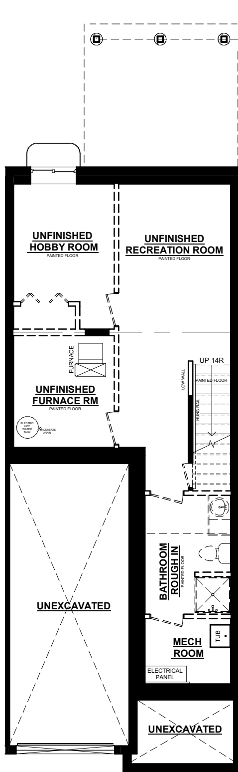
ASHLEE BASEMENT PLAN
