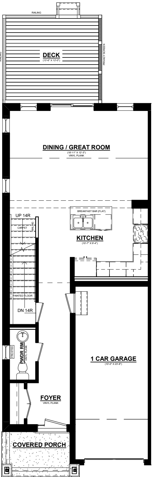
ASHLEE MAINFLOOR PLAN 693 SQ. FT. 8' CEILINGS ON MAINFLOOR
