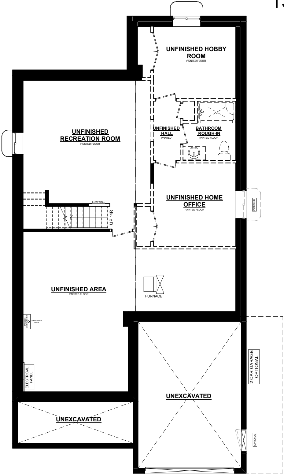
ACADIA 'A' BASEMENT PLAN
