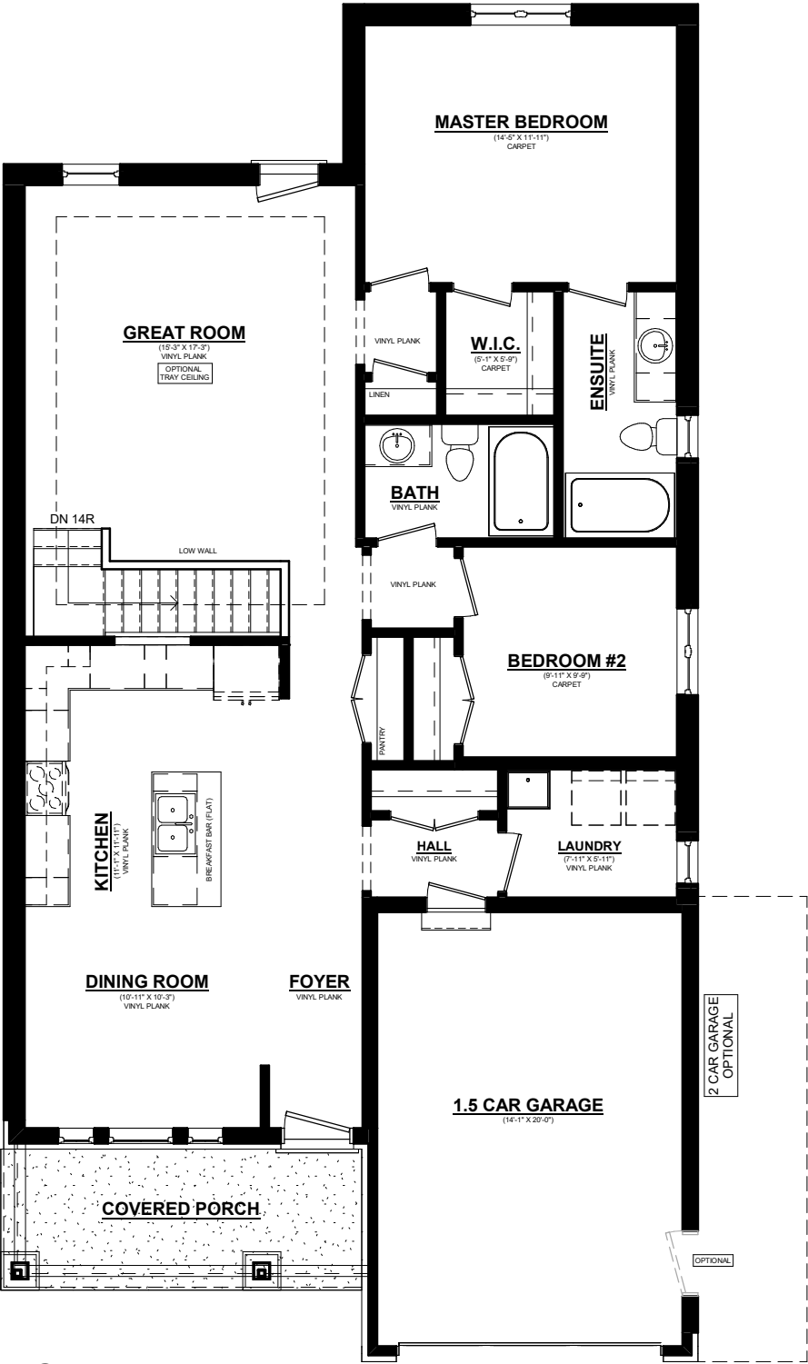
ACADIA 'A' MAIN FLOOR PLAN 1395 SQ. FT. 8' CEILINGS ON MAIN FLOOR
