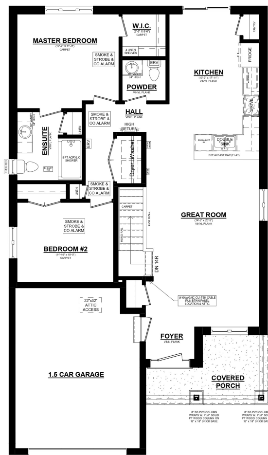
MAYFAIR A MAINFLOOR PLAN 1232 SQ. FT. 8' CEILINGS ON MAINFLOOR
