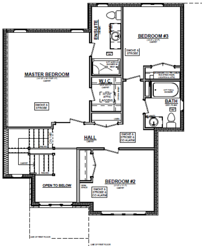
LIVINGSTON B 2ND FLOOR PLAN 908 SQ. FT. (DOES NOT INCLUDE 62 SQ. FT. OPEN TO BELOW) 8' CEILINGS ON 2ND FLOOR
