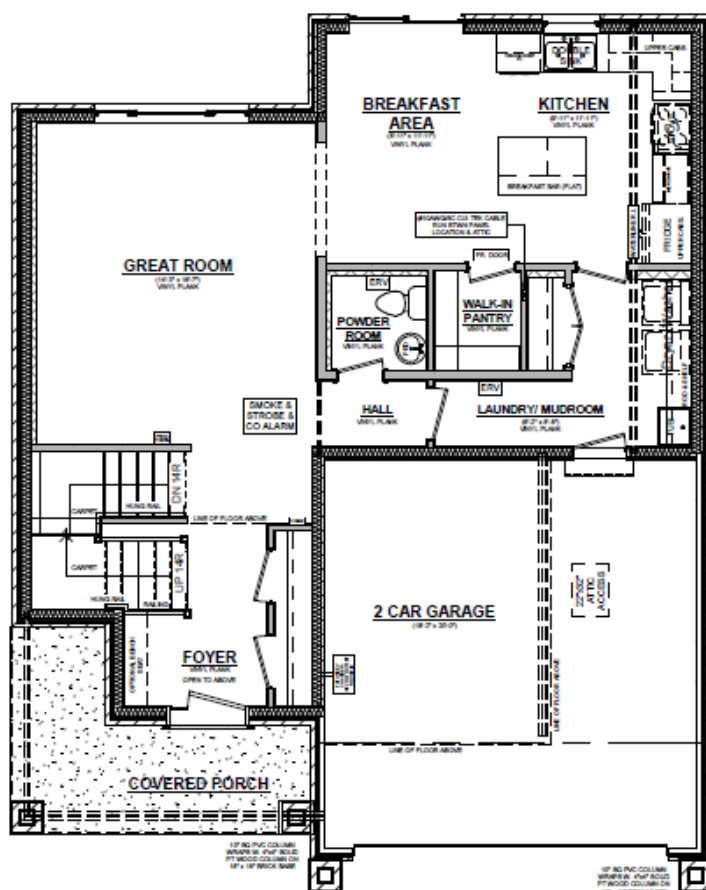
LIVINGSTON B MAIN FLOOR PLAN 939 SQ. FT. 8' CEILINGS ON MAIN FLOOR
