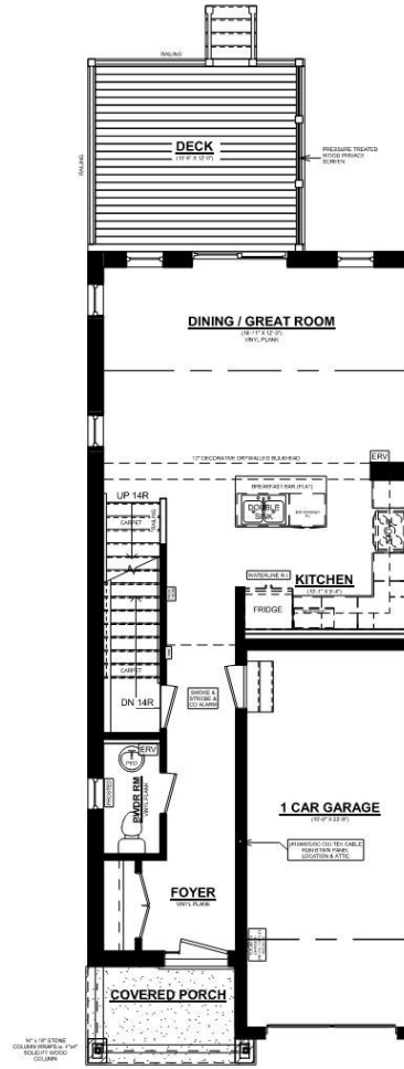
ASHLEE B UNIT #1 MAIN FLOOR PLAN 693 SQ. FT. 8' CEILINGS ON MAIN FLOOR
