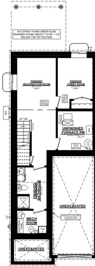
ASHLEE B UNIT #1 BASEMENT PLAN 466 SQ. FT. FINISHED BASEMENT SPACE
