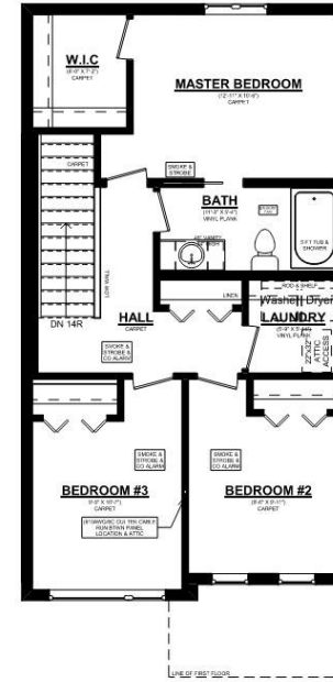
ASHLEE B UNIT #1 2ND FLOOR PLAN 704 SQ. FT. 8' CEILINGS ON 2ND FLOOR
