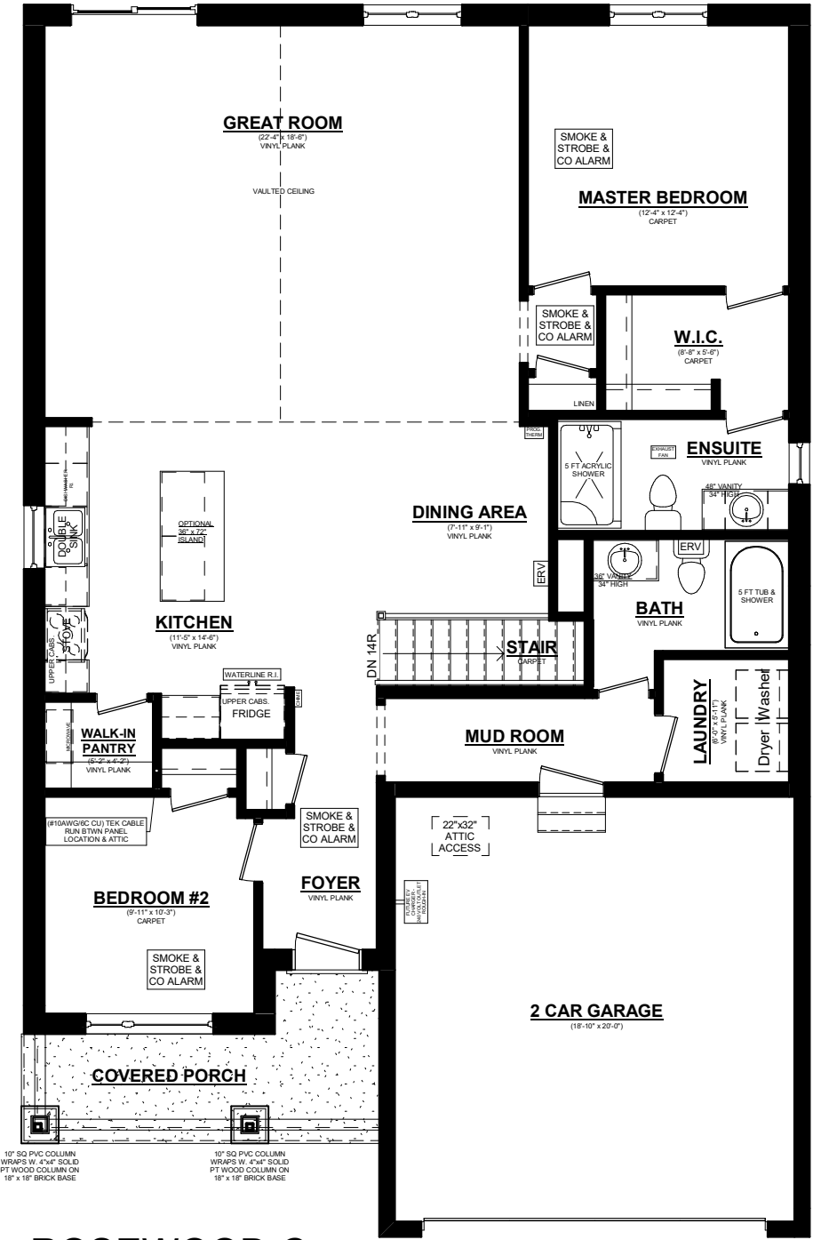
ROSEWOOD C MAINFLOOR PLAN 1543 SQ. FT. 8' CEILINGS ON MAINFLOOR
