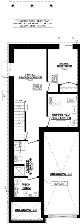
ASHLEE B BASEMENT PLAN 466 SQ. FT. FINISHED BASEMENT SPACE
