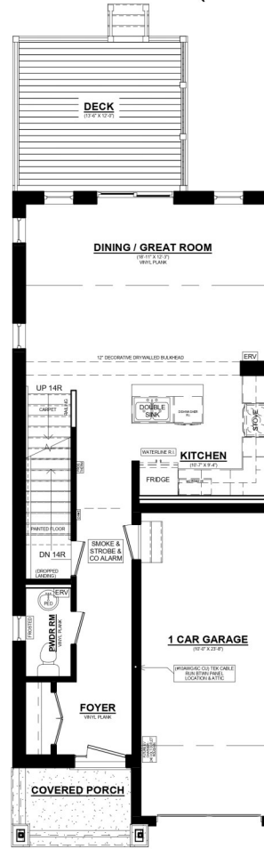
ASHLEE B MAINFLOOR PLAN 693 SQ. FT. 8' CEILINGS ON MAINFLOOR
