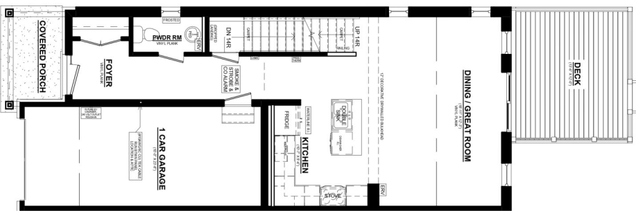
ASHLEE C MAIN FLOOR PLAN 693 SQ. FT. 8' CEILINGS ON MAIN FLOOR
