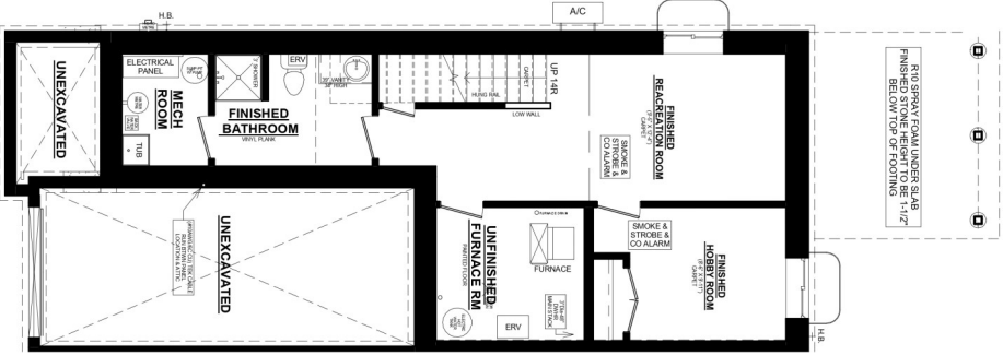
ASHLEE C BASEMENT PLAN 466 SQ. FT. FINISHED BASEMENT SPACE
