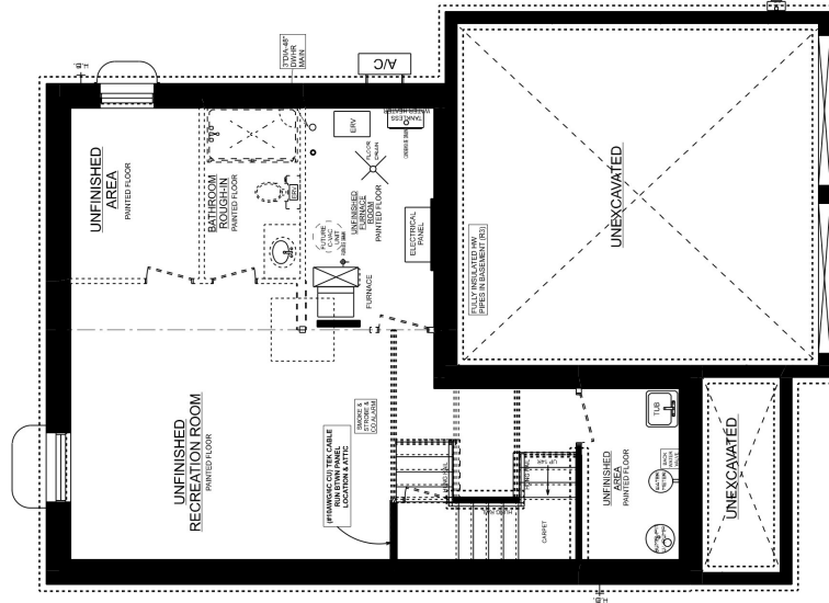
MAPLERIDGE 'A' BASEMENT PLAN
