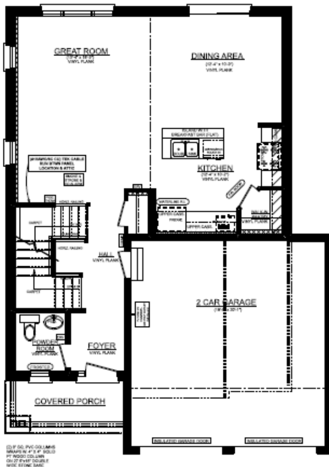
MAPLERIDGE 'A' MAINFLOOR PLAN 797 SQ. FT. 2 CAR GARAGE 8' CEILINGS ON MAINFLOOR
