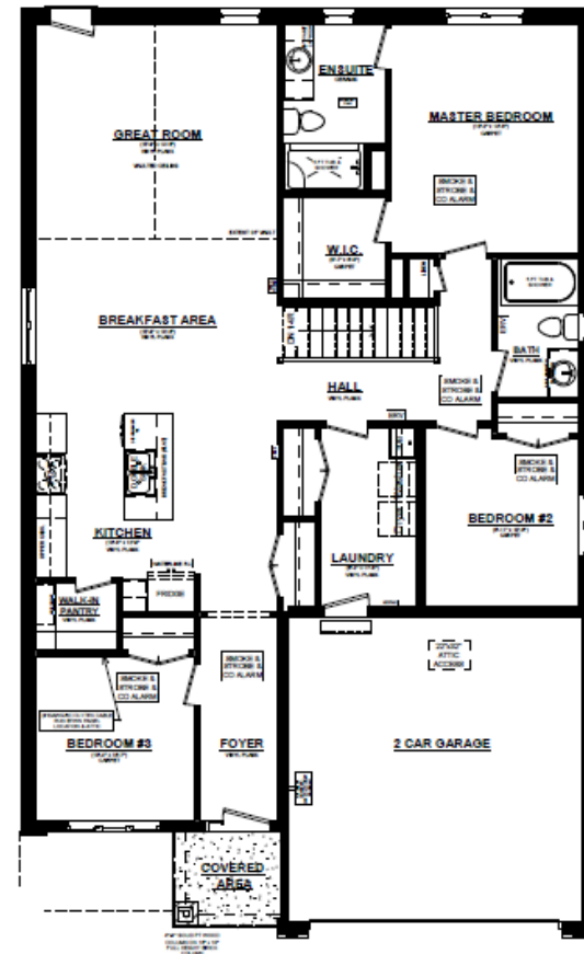
DUNMOOR C MAINFLOOR ELEVATION 1884 SQ. FT. 8' CEILINGS ON MAINFLOOR
