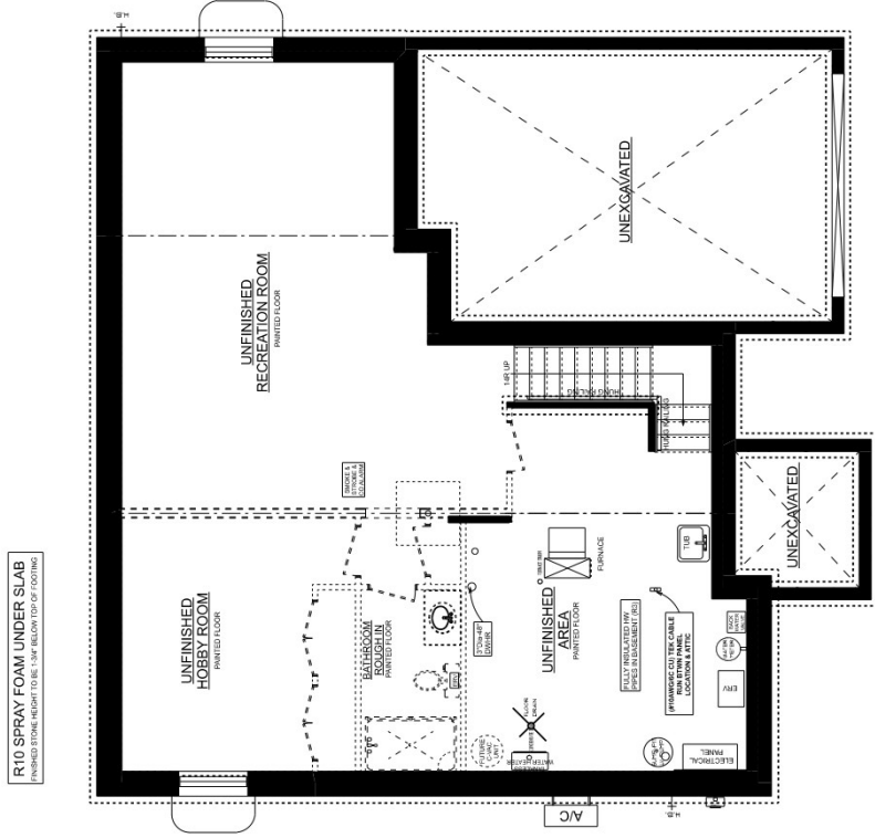
THE KNOLLWOOD 'C' BASEMENT PLAN
