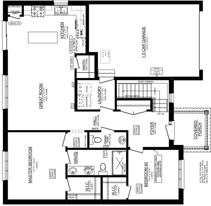
THE KNOLLWOOD 'C' MAIN FLOOR PLAN 1229 SQ. FT. 8' CEILINGS ON MAIN FLOOR
