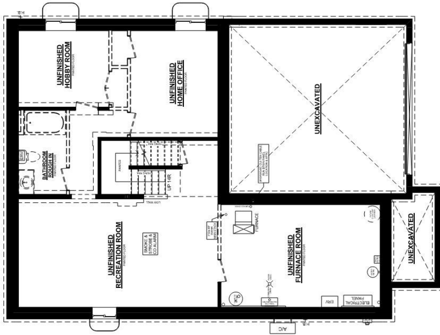
STONEHAVEN C BASEMENT PLAN
