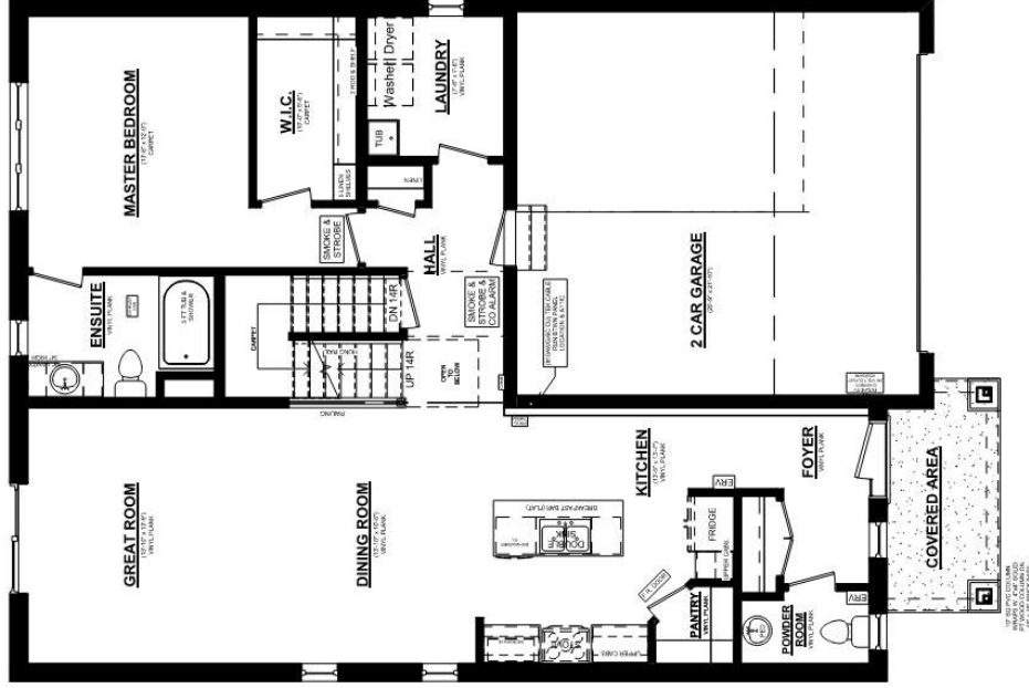
STONEHAVEN C MAINFLOOR ELEVATION 1313 SQ. FT. 8" CEILINGS ON MAINFLOOR
