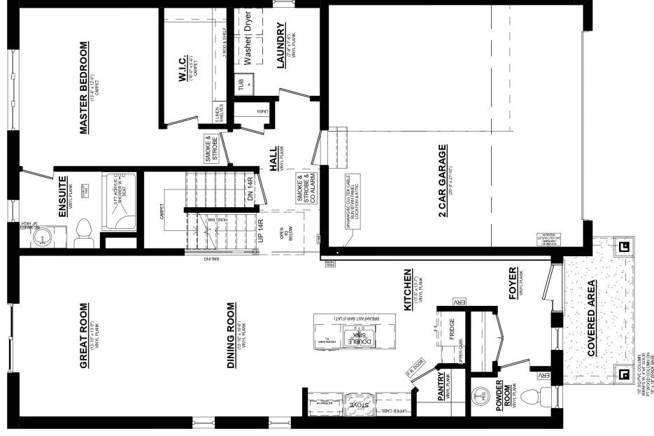
STONEHAVEN C MAINFLOOR ELEVATION
