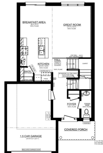
ASPEN 'B' MAINFLOOR PLAN 8' CEILINGS ON MAINFLOOR 700 SQ. FT. PRELIMINARY PLAN/NOT FOR CONSTRUCTION
