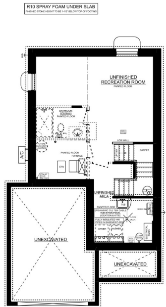
ASPEN 'B' BASEMENT PLAN PRELIMINARY PLAN/NOT FOR CONSTRUCTION
