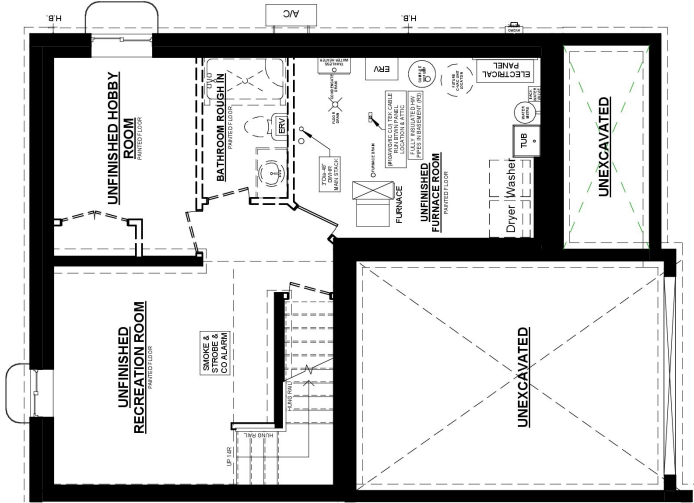
ELMWOOD A UNIT #2 BASEMENT PLAN
