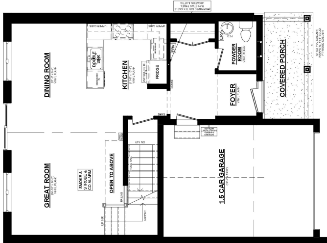
ELMWOOD A UNIT #2 MAINFLOOR PLAN 745 SQ. FT. 8' CEILINGS ON MAINFLOOR
