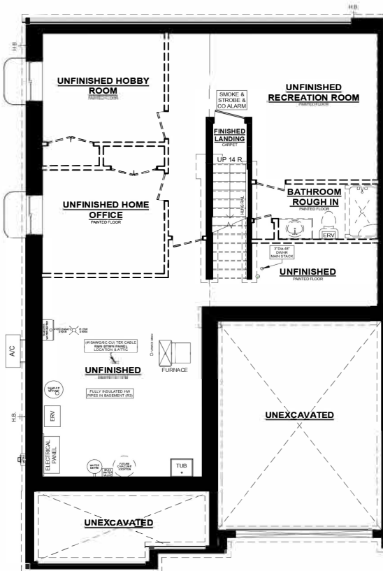
EASTON A UNIT #1 BASEMENT PLAN
