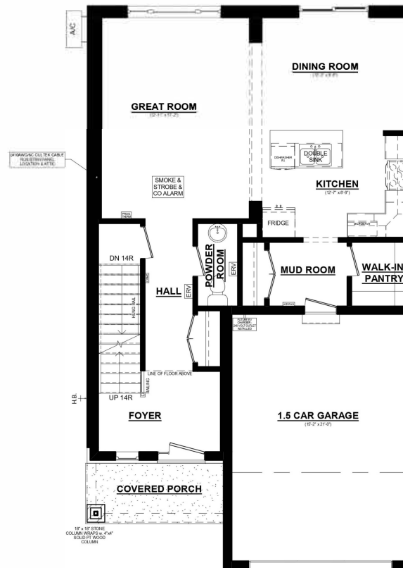
SEDONA 'B' UNIT #1 MAIN FLOOR PLAN 879 SQ. FT. 8' CEILINGS ON MAIN FLOOR
