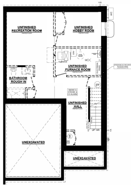
SEDONA 'B' UNIT #2 BASEMENT PLAN
